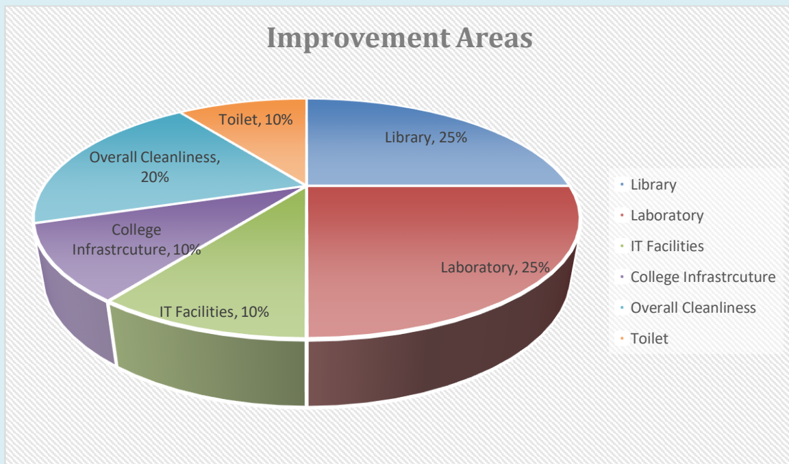
Figure 8: Improvement Percentage
